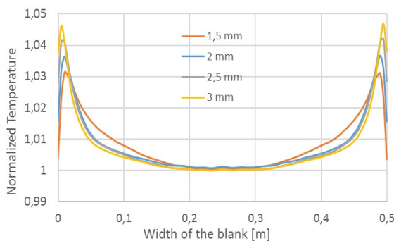
Fig. 17: Temperature in x-direction in the centre
