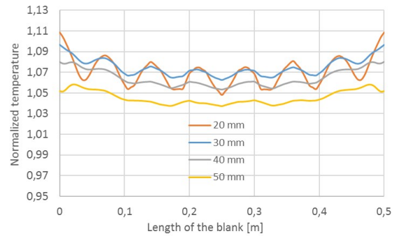
Fig. 12: Temperature in z-direction at the edge
