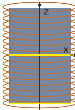
Fig. 2: Evaluation path in x-direction
