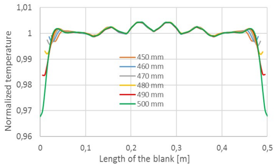
Fig. 15: Temperature in z-direction in the centre
