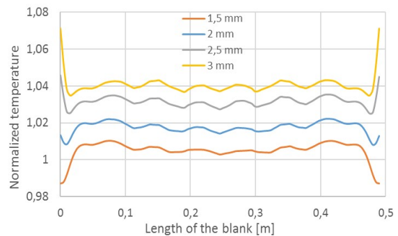
Fig. 20: Temperature in z-direction at the edge
