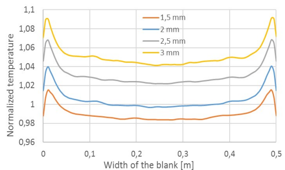
Fig. 18: Temperature in x-direction at the end
