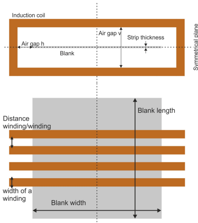
Fig. 1: Sketch of the numerical model
