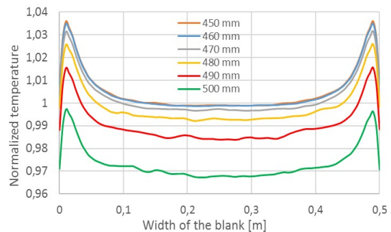
Fig. 14: Temperature in x-direction at the end
