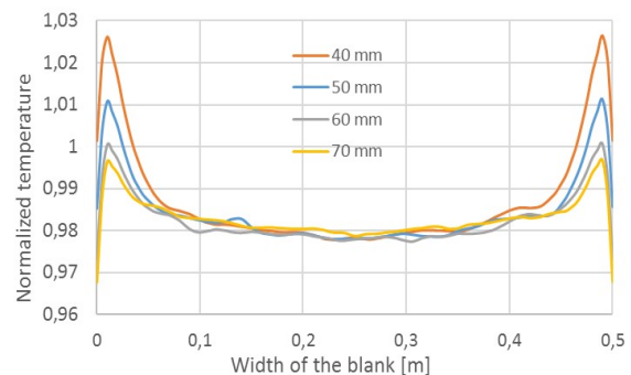
Fig. 5: Temperature in x-direction at the end
