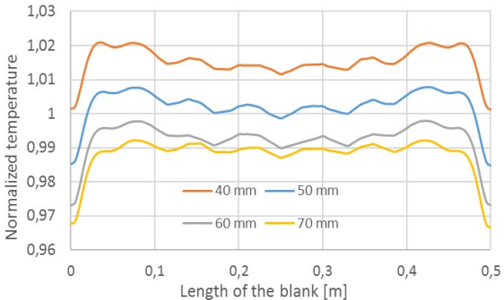
Fig. 8: Temperature in z-direction at the edge
