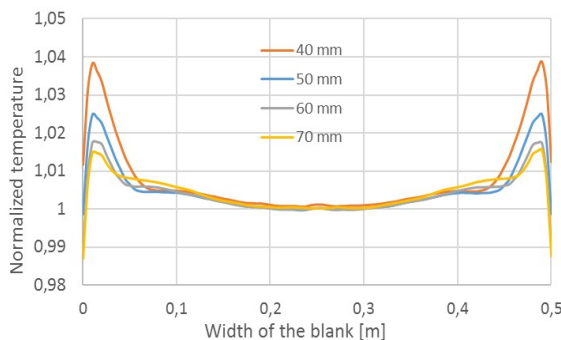
Fig. 4: Temperature in x-direction in the centre
