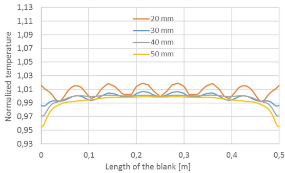
Fig. 11: Temperature in z-direction in the centre
