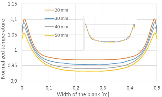
Fig. 10: Temperature in x-direction at the end
