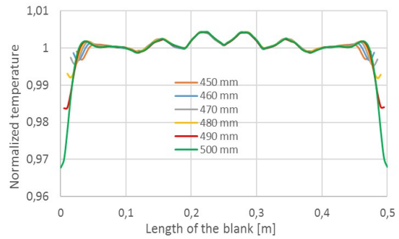
Fig. 16: Temperature in z-direction at the edge
