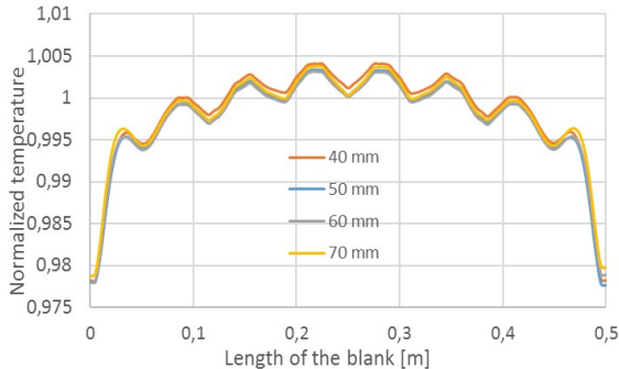
Fig.7: Temperature in z-direction in the centre
