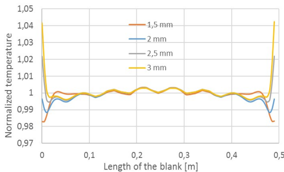
Fig. 19: Temperature in z-direction in the centre
