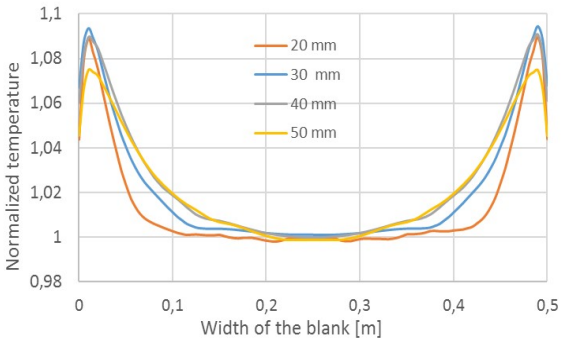
Fig. 9: Temperature in x-direction in the centre
