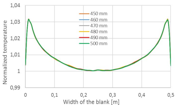
Fig. 13: Temperature in x-direction in the centre
