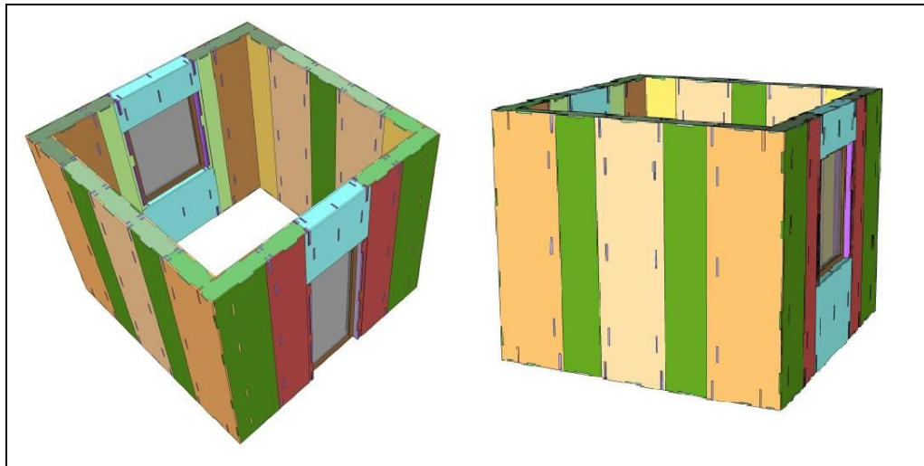
Figure 4. Plywood frame structure installation design (type D)
