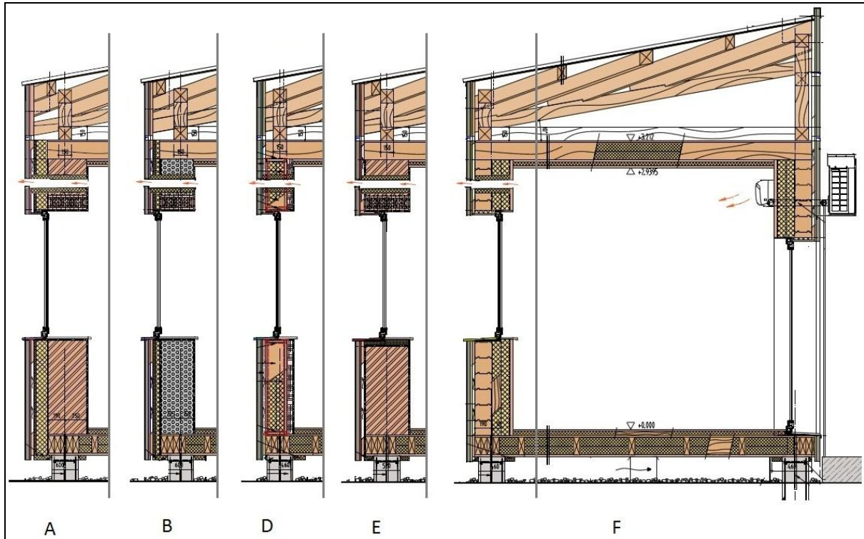
Figure 5. The experimental construction design and engineering solutions in cross section (type A, B, D, E, F)
